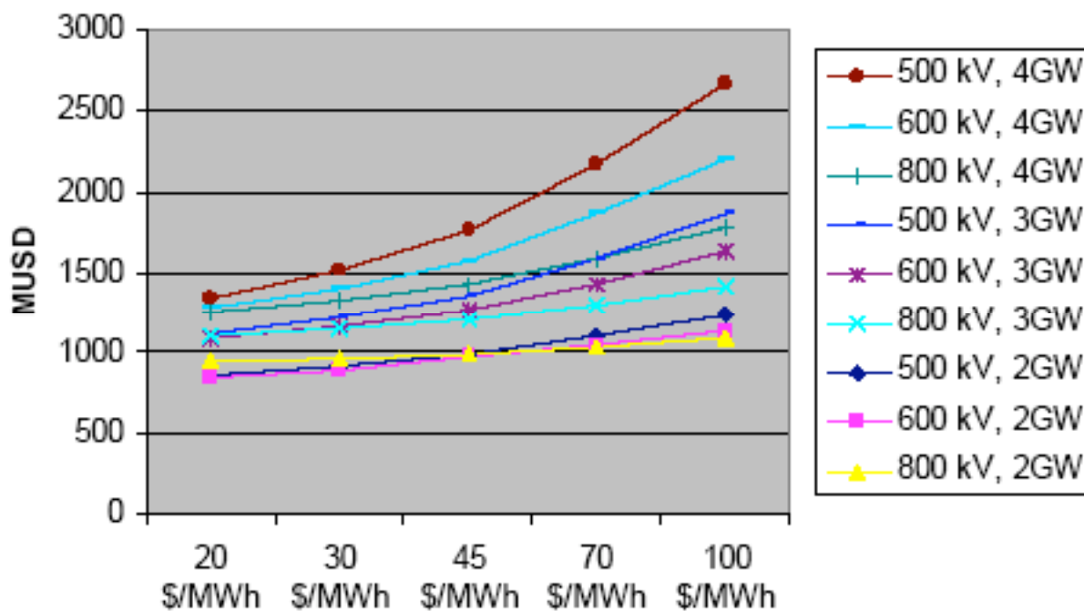
Fig. 6 Total cost as a function of Value of Losses
